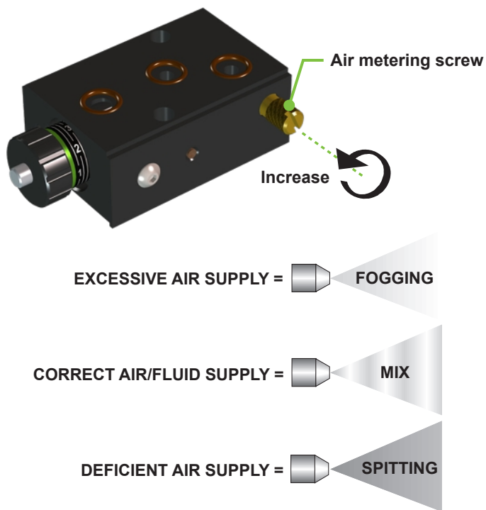
Figure 34: Adjusting airflow
