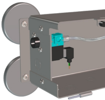
Figure 19: Magnet mount
