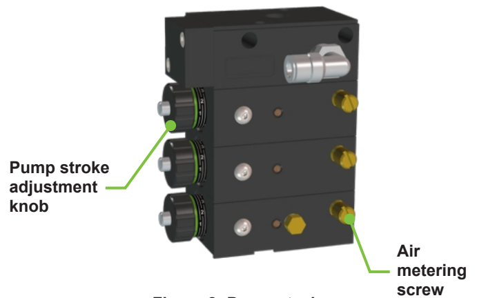
Figure 2: Pump stack
