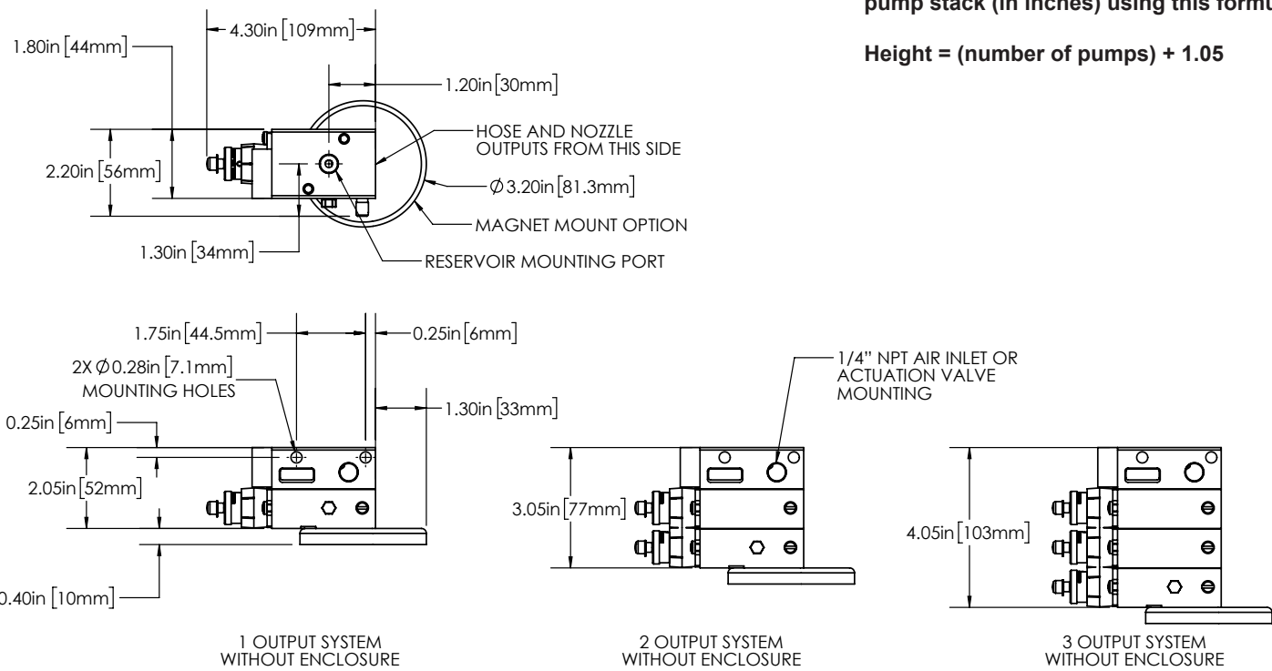
Figure 17: Systems without enclosures
