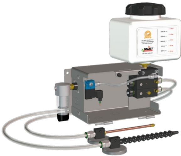
Figure 4: Multiple pump output system with an enclosure
