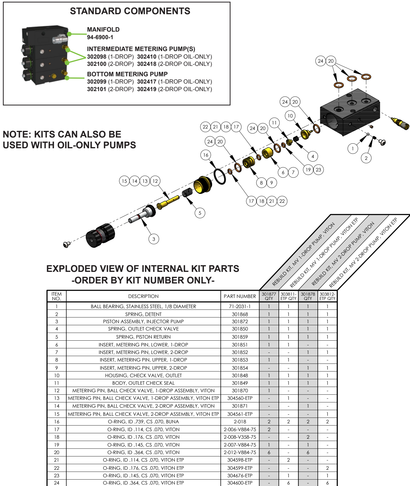
Figure 46: MV pump components
