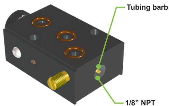
Figure 9: Outlet port
