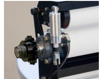
Rollers synchronized to sheet feed drive.
